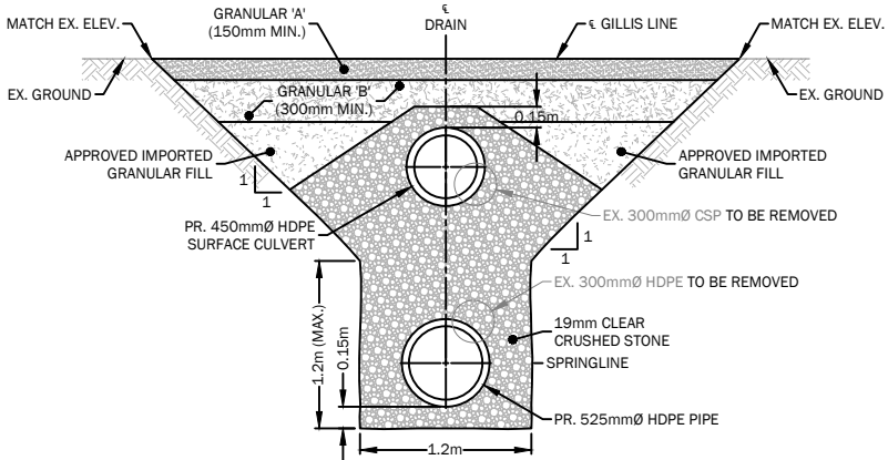
'B' DRAIN OF THE WEST MCTAGGART DRAIN GILLIS LINE CROSSING SECTION
