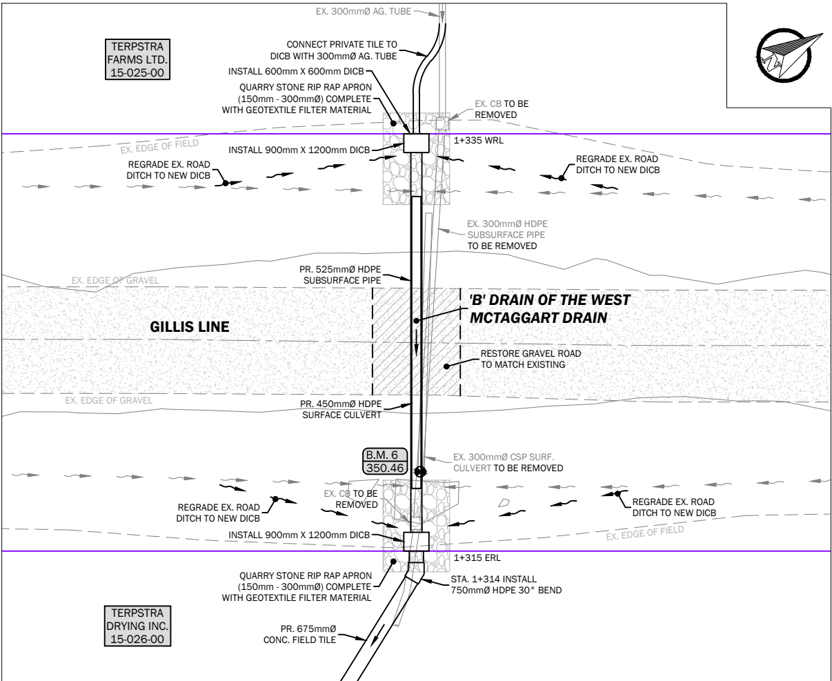
'B' DRAIN OF THE WEST MCTAGGART DRAIN GILLIS LINE CROSSING DETAIL
