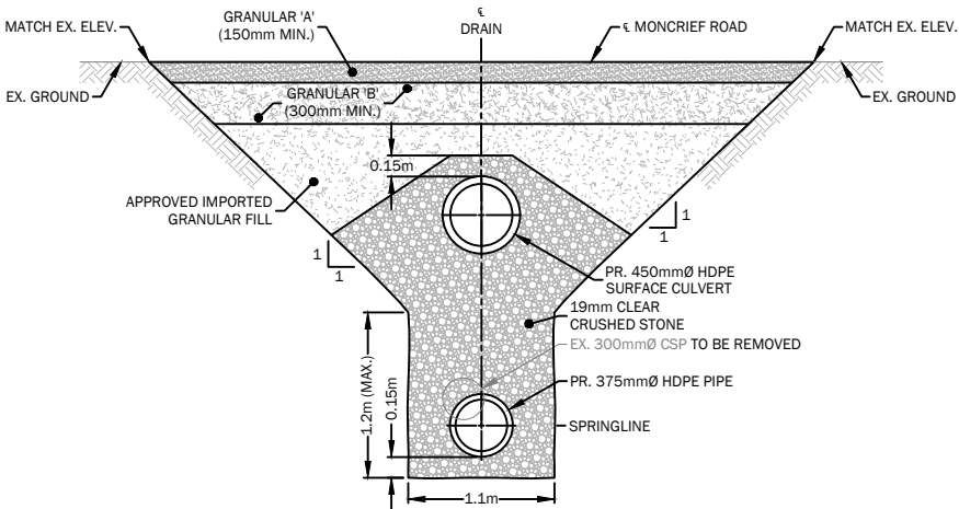
'A' DRAIN OF THE CLARK DRAIN MONCRIEF ROAD CROSSING SECTION
