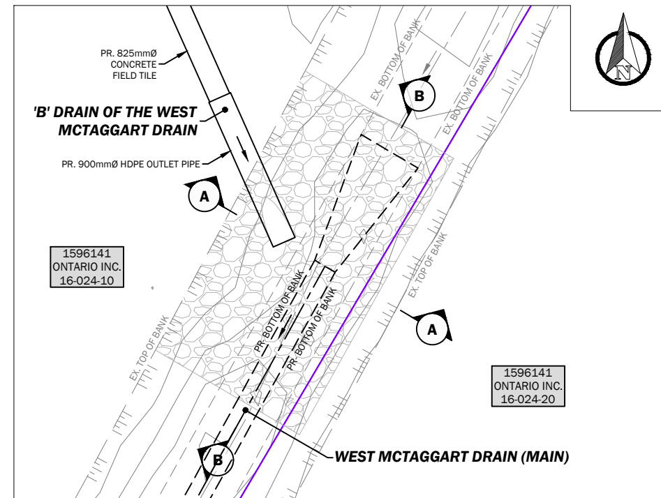
'B' DRAIN OF THE WEST MCTAGGART DRAIN OUTLET DETAIL
