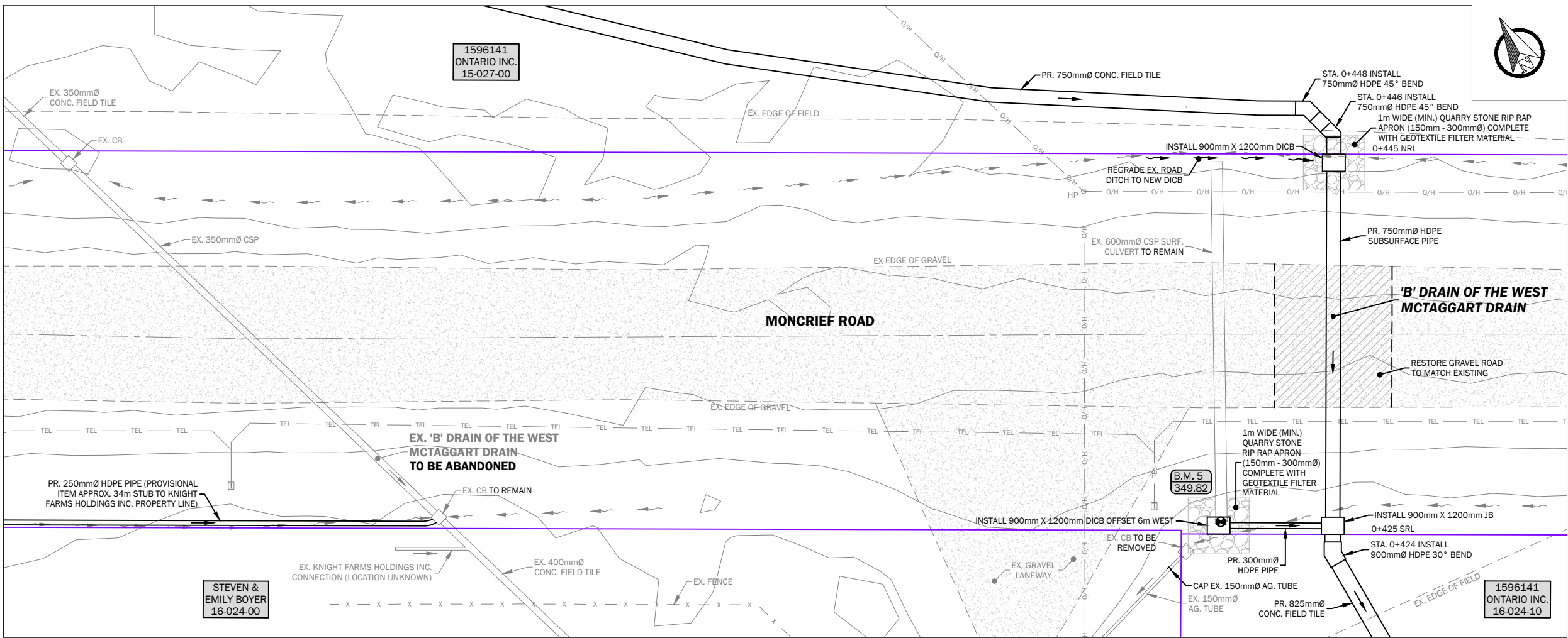
'B' DRAIN OF THE WEST MCTAGGART DRAIN MONCRIEF ROAD CROSSING DETAIL
