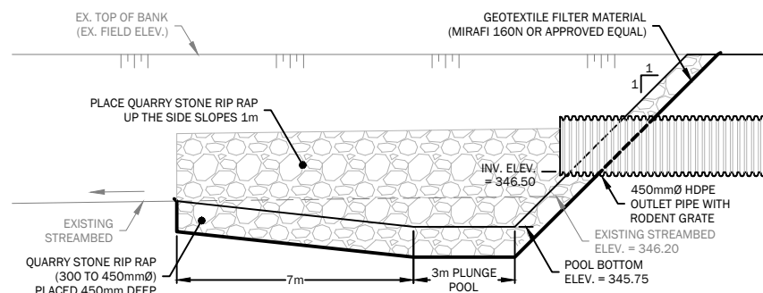
'A' DRAIN OF THE CLARK DRAIN PLUNGE POOL DETAIL N.T.S.
