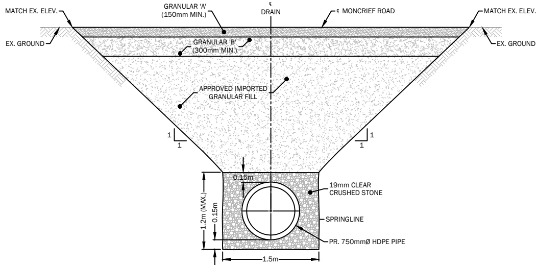
'B' DRAIN OF THE WEST MCTAGGART DRAIN MONCRIEF ROAD CROSSING SECTION N.T.S.
