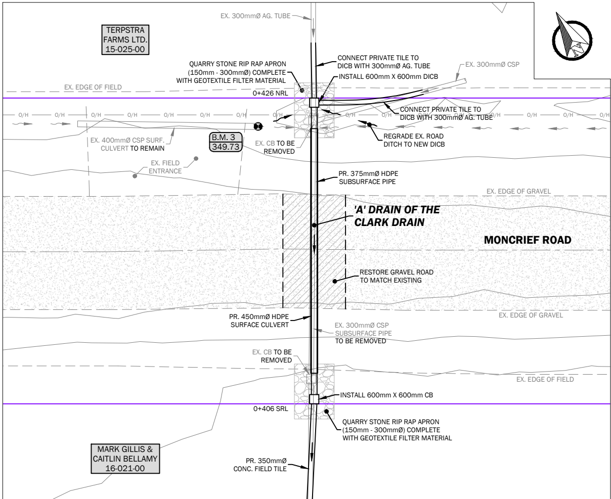
'A' DRAIN OF THE CLARK DRAIN MONCRIEF ROAD CROSSING DETAIL
