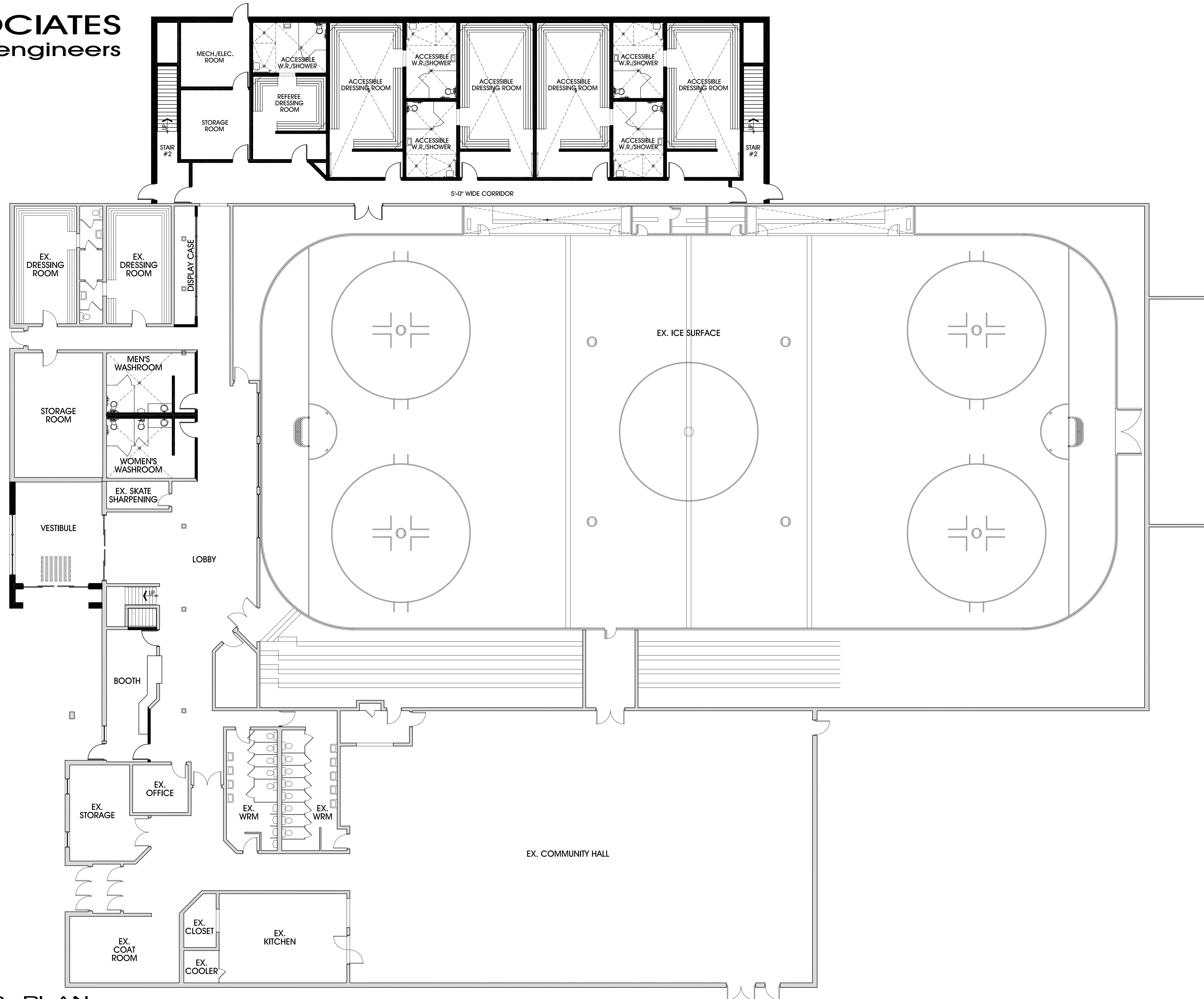
GROUND FLOOR PLAN SCALE: 3/32" = 1'-0"
